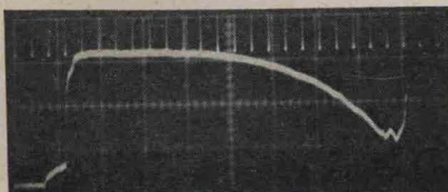
FIG. 3. (a) The oscillograph is of a voltage developed across a 3\ \Omega gauge during a cycle of the supply. The scale is 10\ \mu\text{sec}/\text{div} . (b) Voltage-time record of a 38 kilobar final state shock wave in 6061-T6 aluminum. The scale is 0.5\ \mu\text{sec}/\text{div} .
