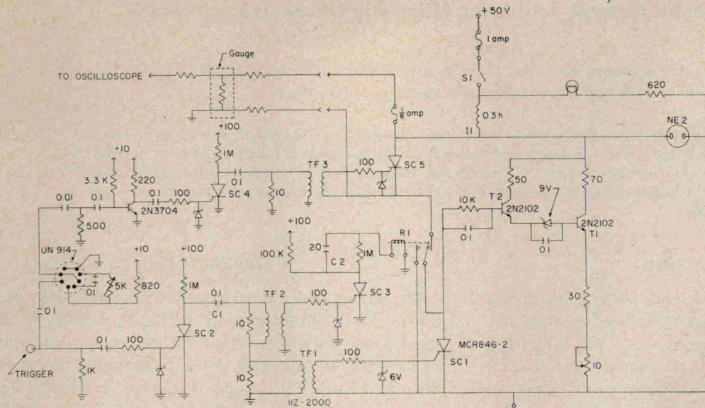
FIG. 2. Schematic of manganin gauge constant current supply.
